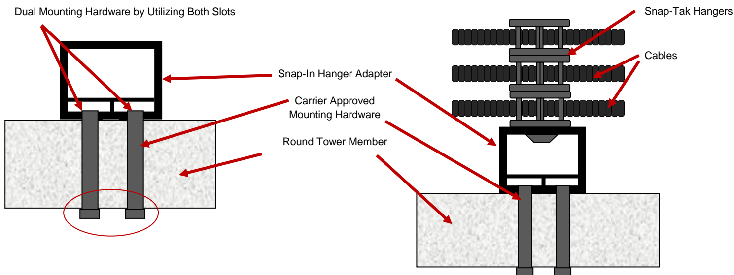
Configuration showing snap-in hanger adapter securely attached to tower member to support up to 3 Snap-Tak Hangers.
