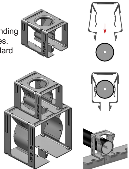
SIC Clamps shown with Coax and tower standoff
